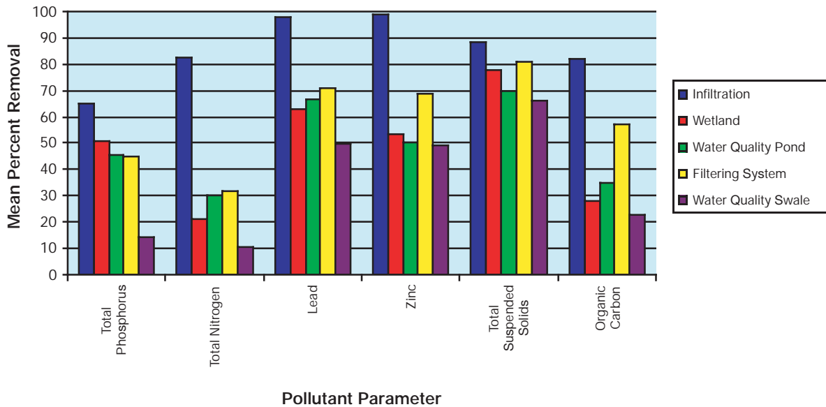
Infiltration vs. Other Stormwater BMPs
